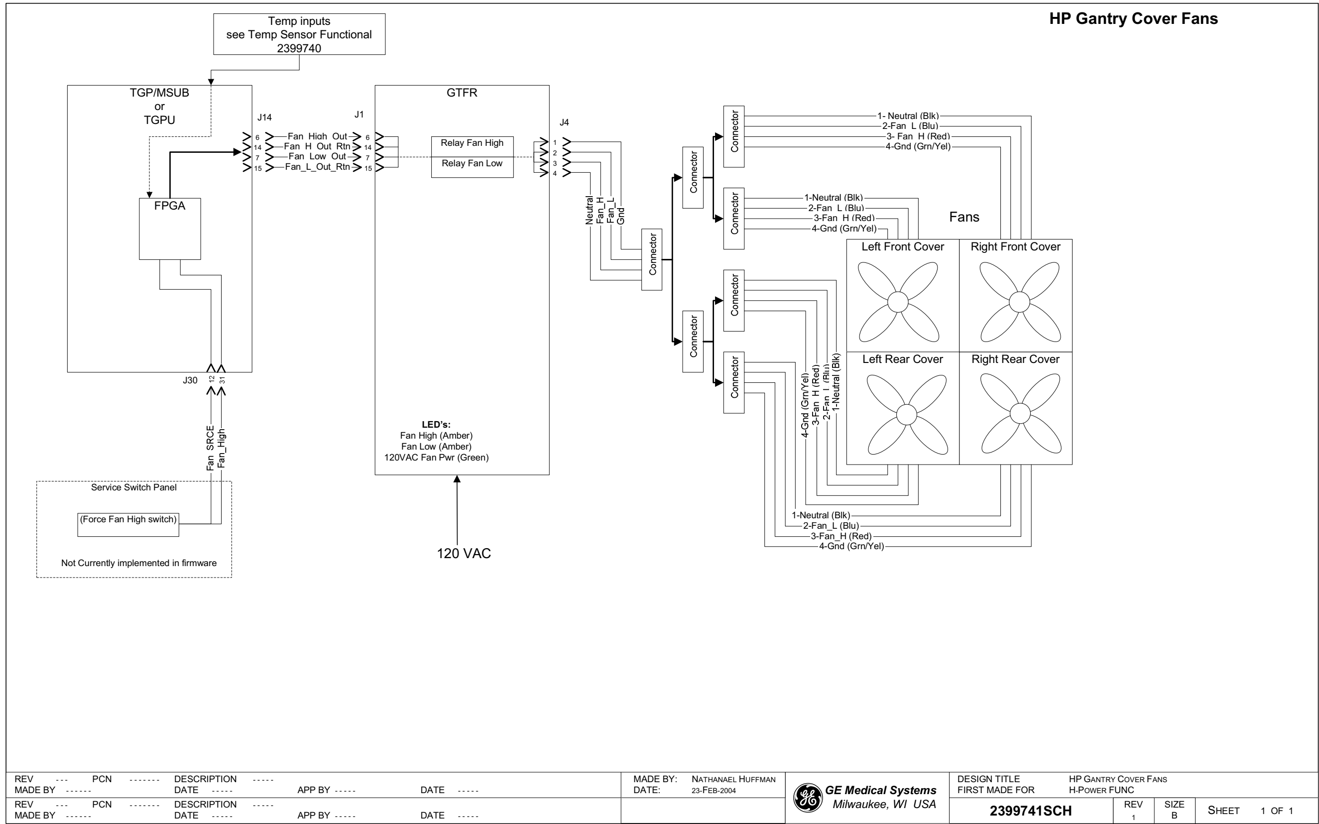
Figure 7-2 2399741 Sheet 1, Rev. 1
