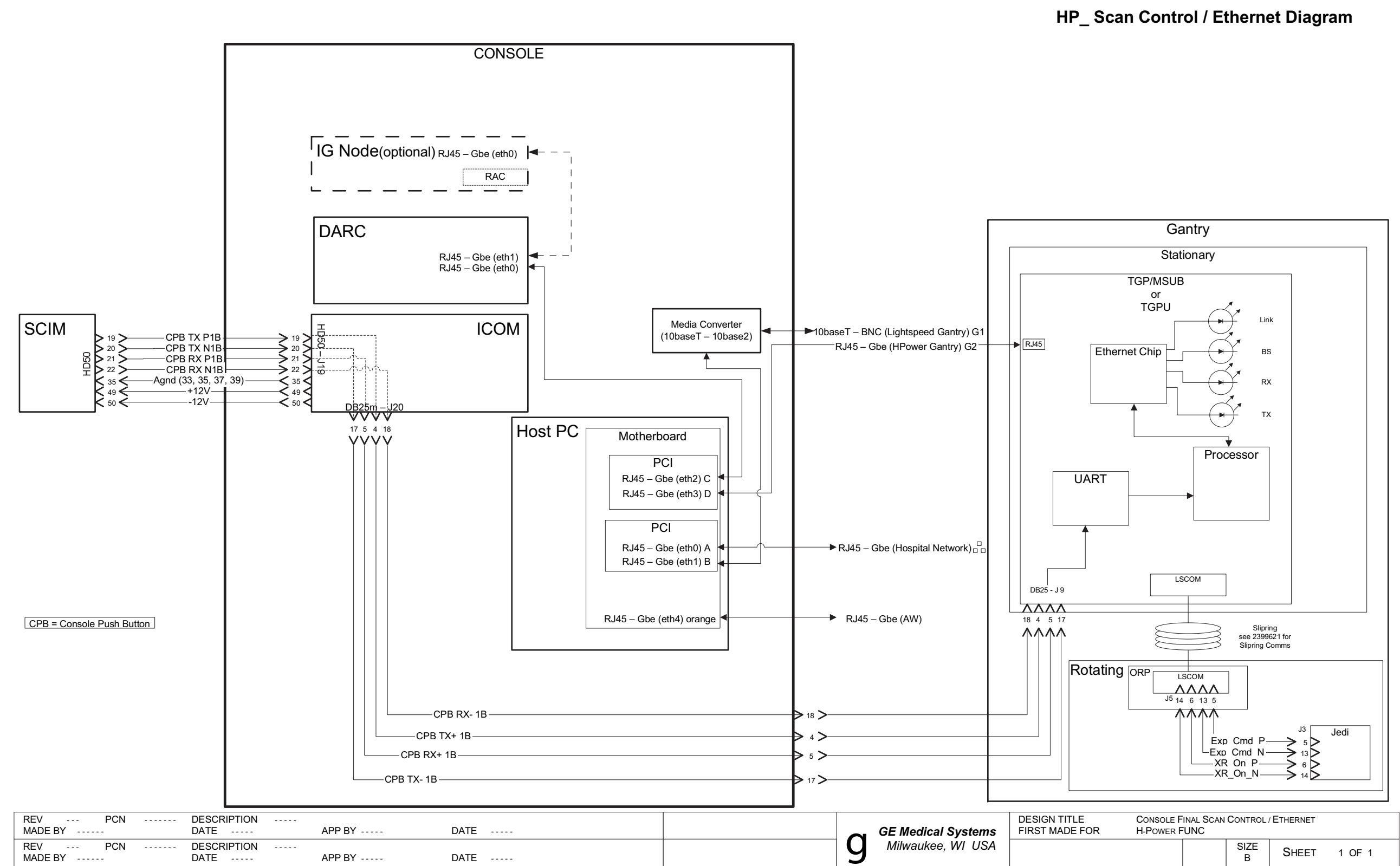
Figure 1-2 2399622 Sheet 1, Rev 1
