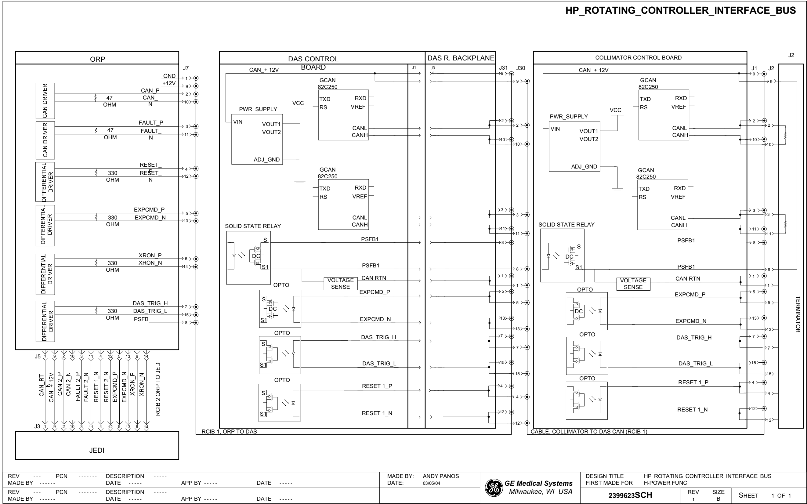
Figure 1-3 2399623 Sheet 1, Rev. 1
