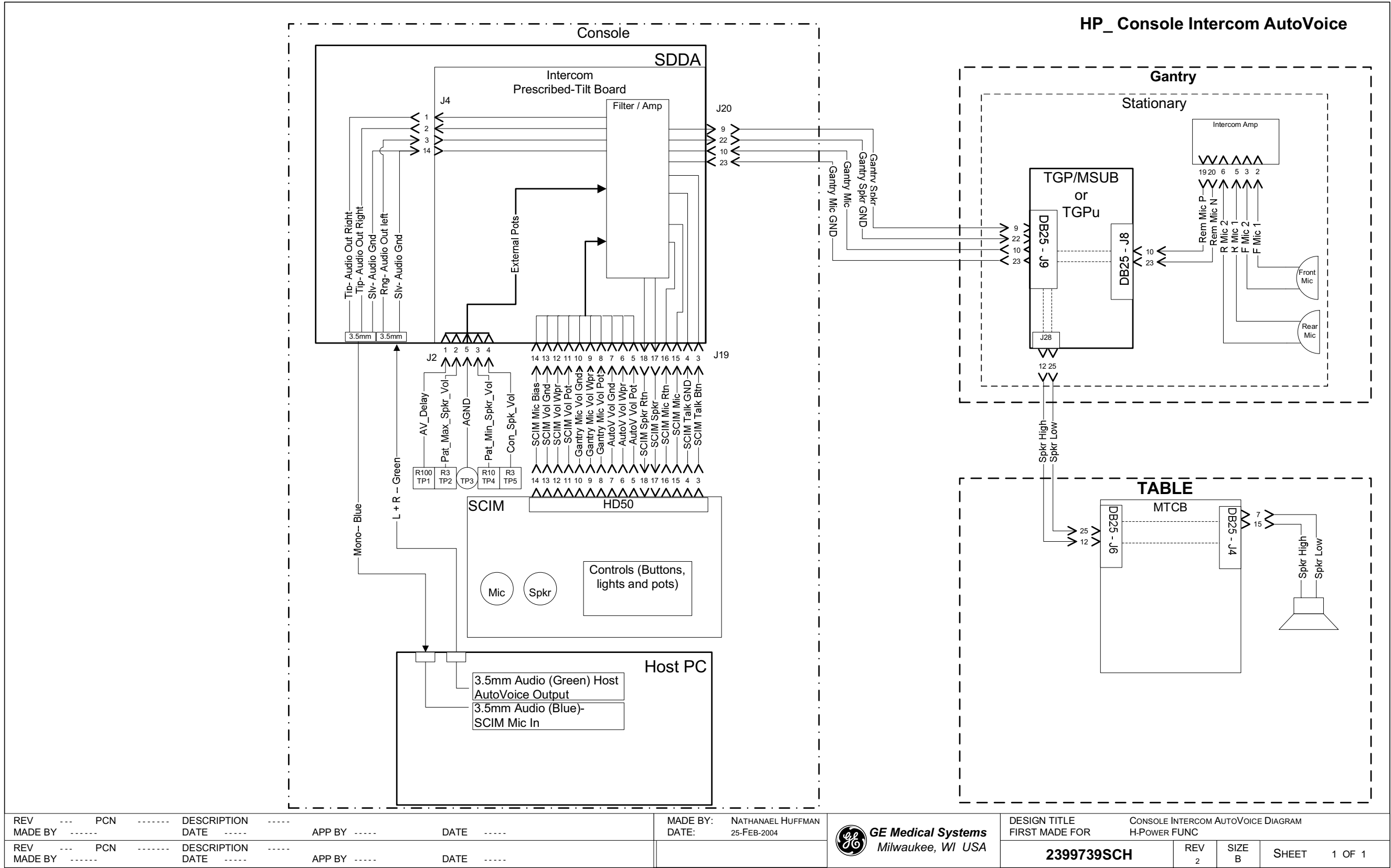
Figure 6-6 2399739 Sheet 1, Rev. 2
