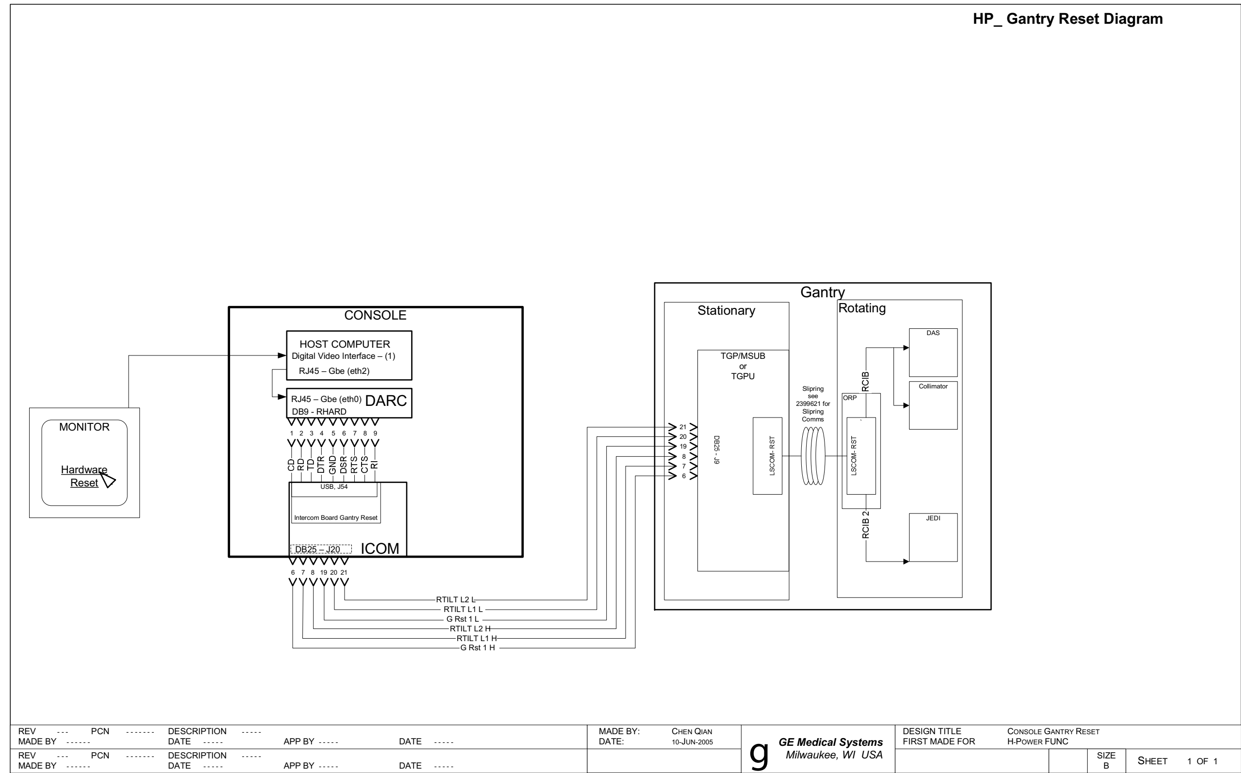
Figure 6-2 2399734 Sheet 1, Rev. 1
