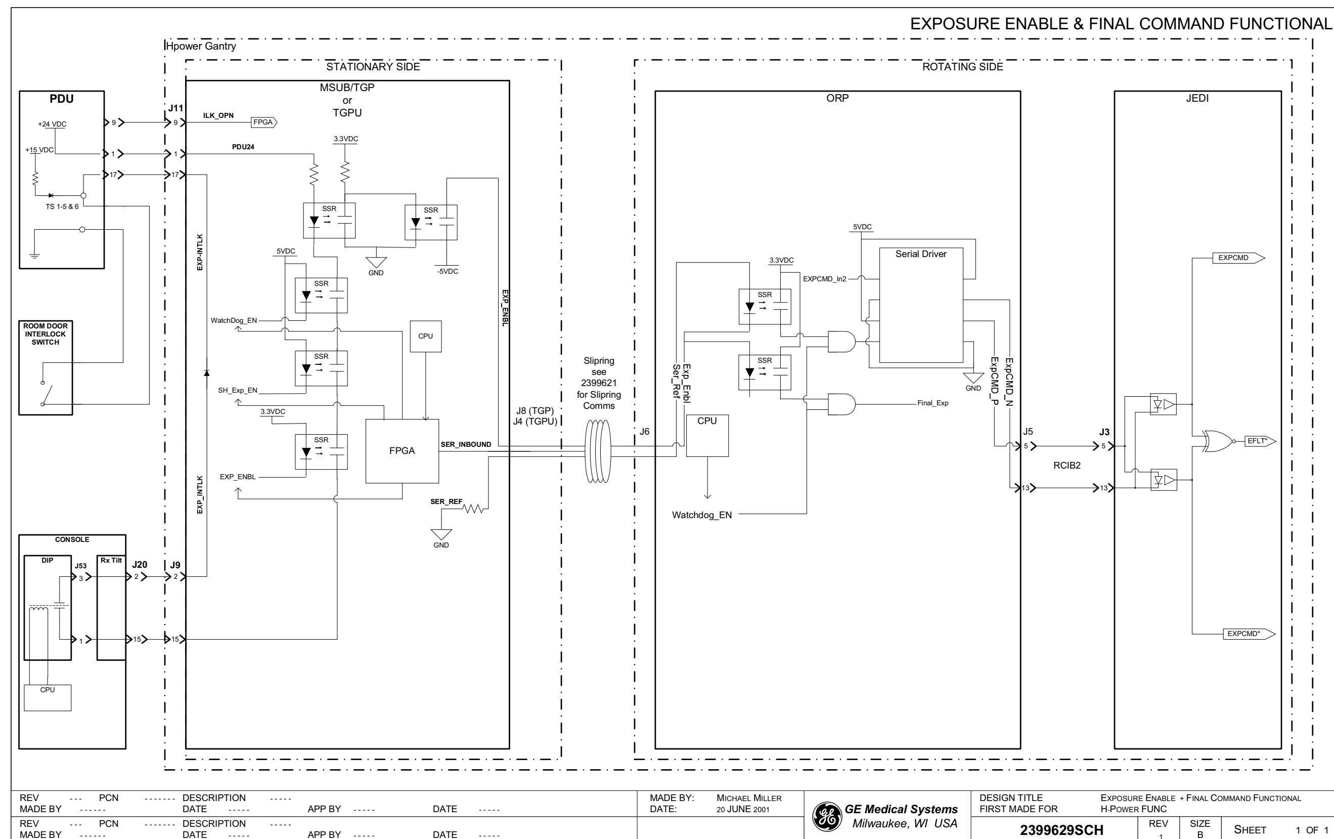
Figure 2-5 2399629 Sheet 1, Rev. 1
