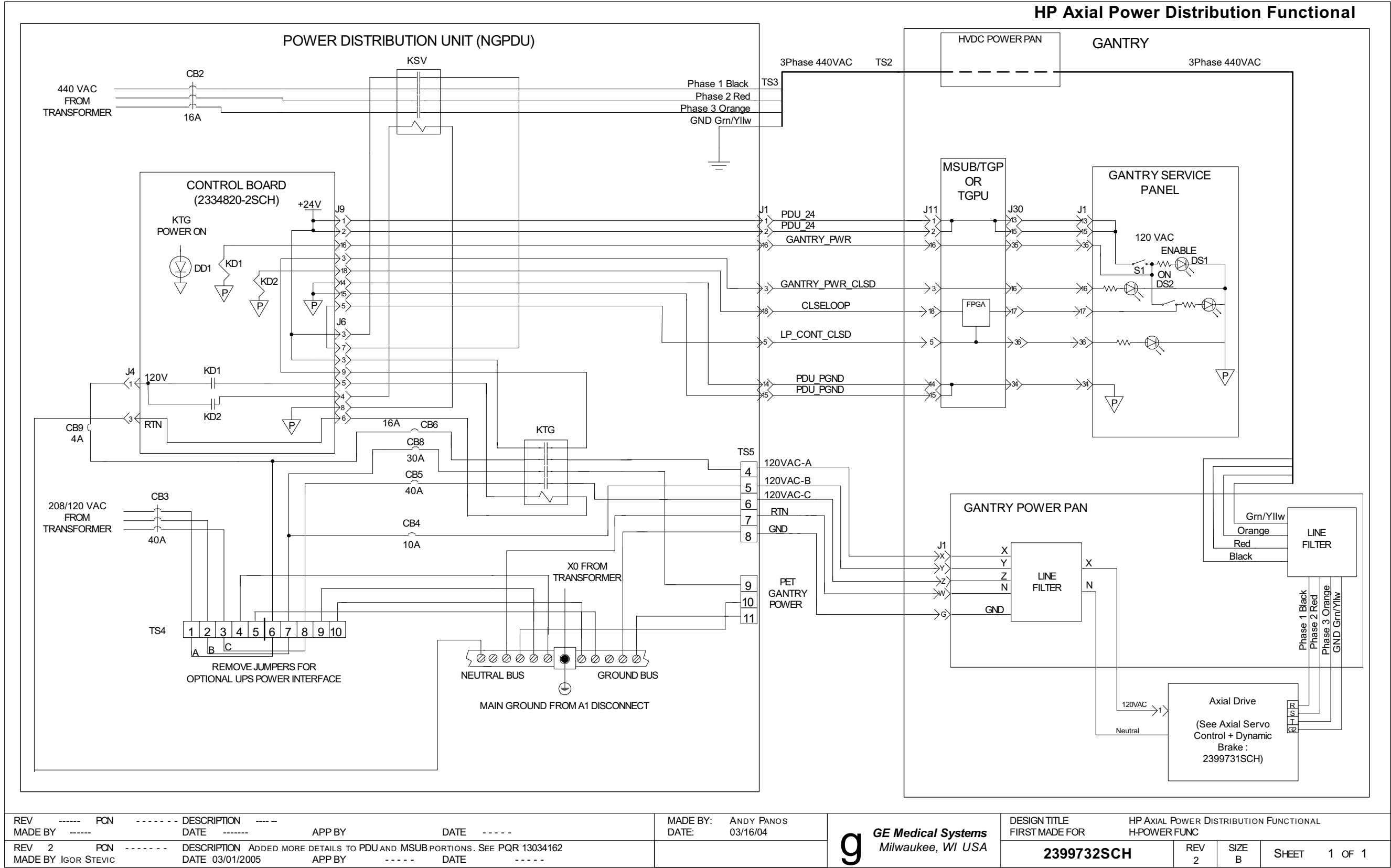
Figure 5-2 2399732 Sheet 1 Rev. 2
