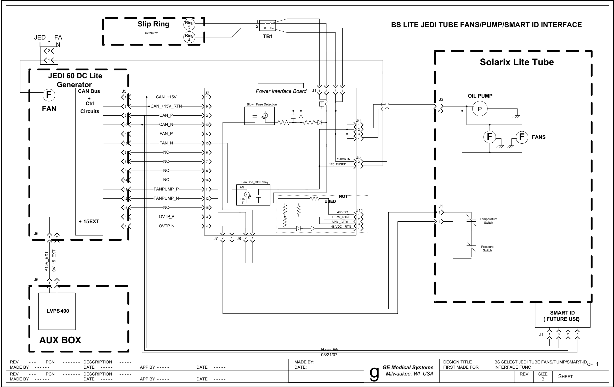
Figure 2-1 2399624 Sheet 1, Rev. 1
