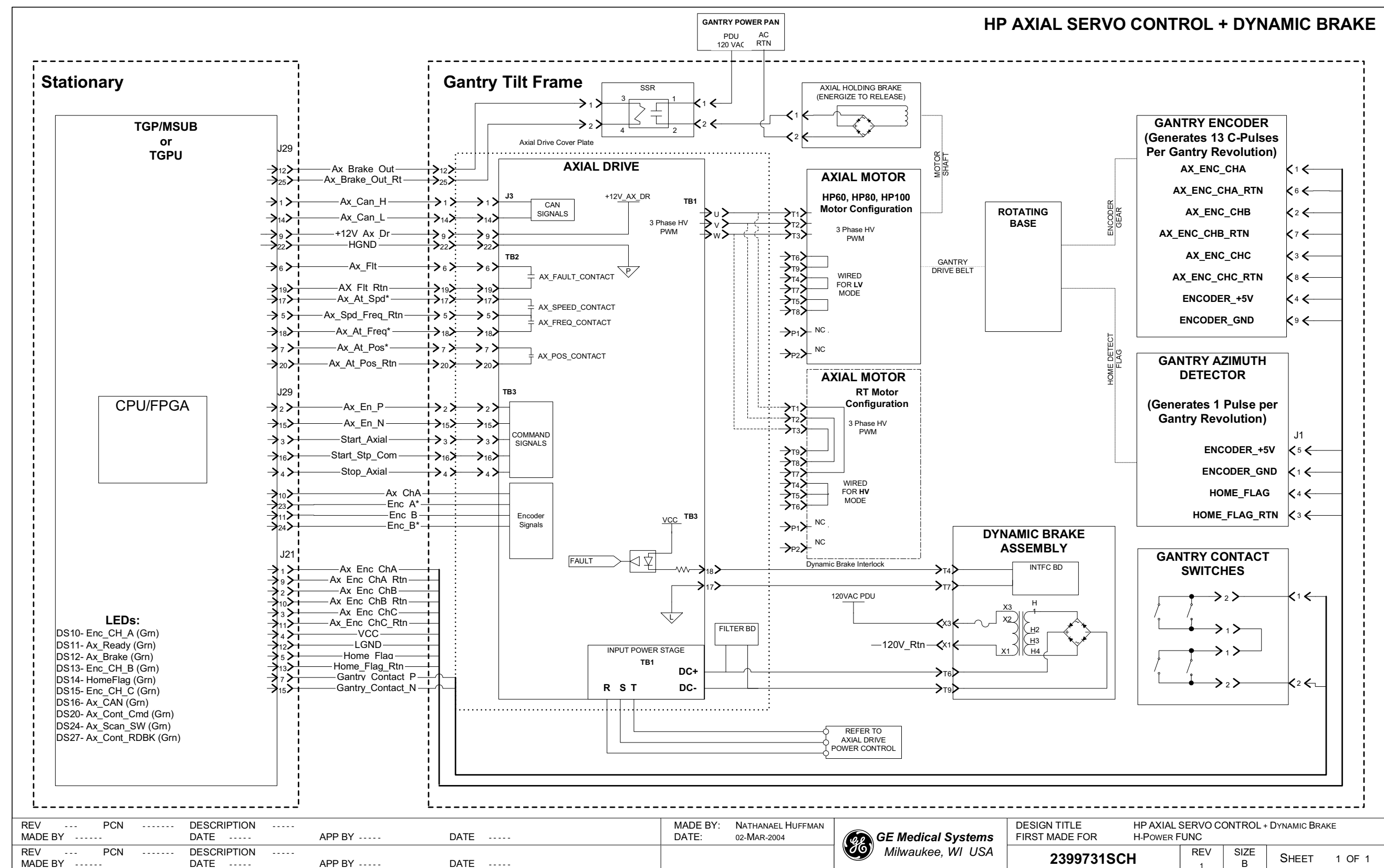
Figure 5-1 2399731 Sheet 1 Rev. 1
