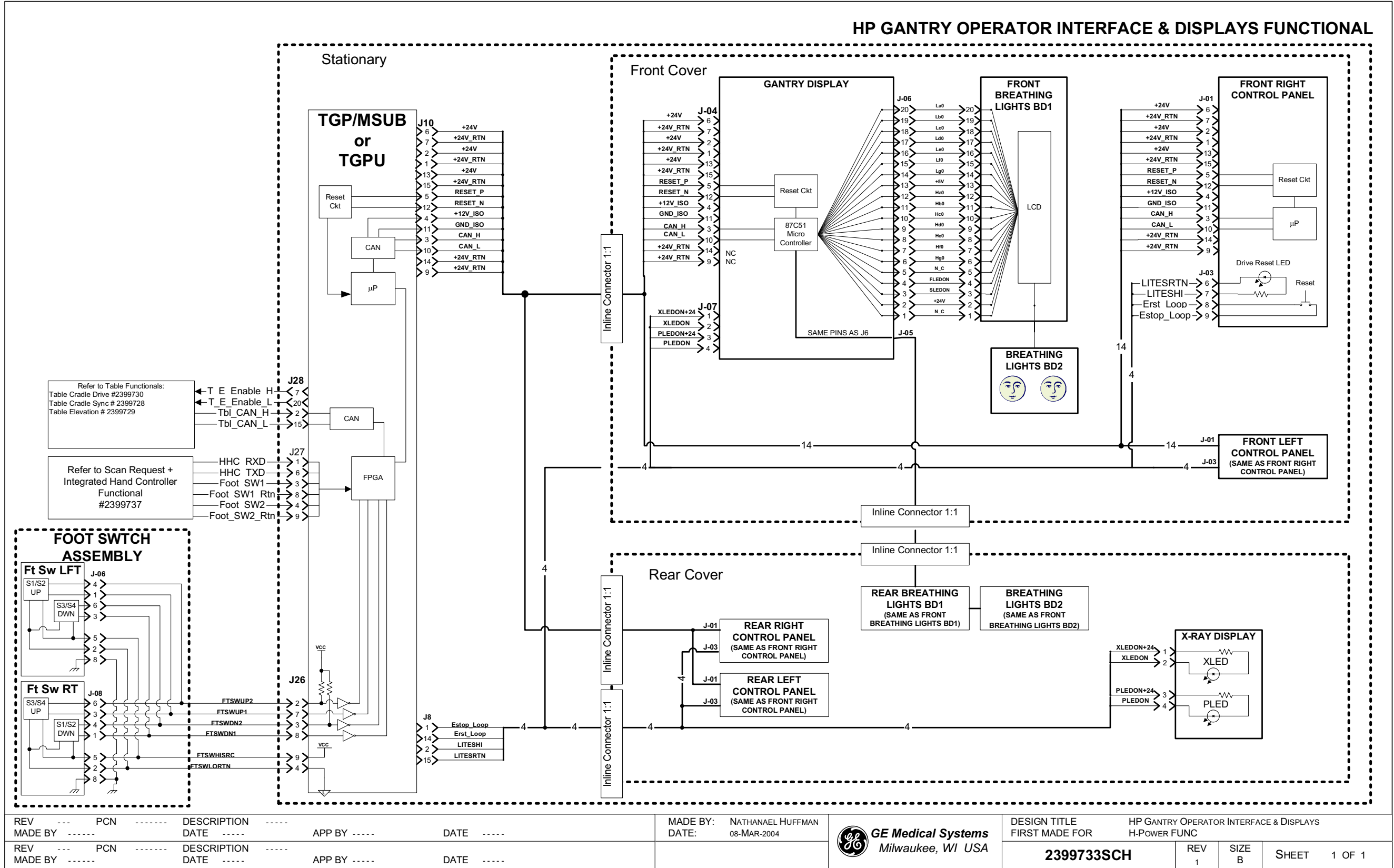
Figure 6-1 2399733 Sheet 1, Rev. 1
