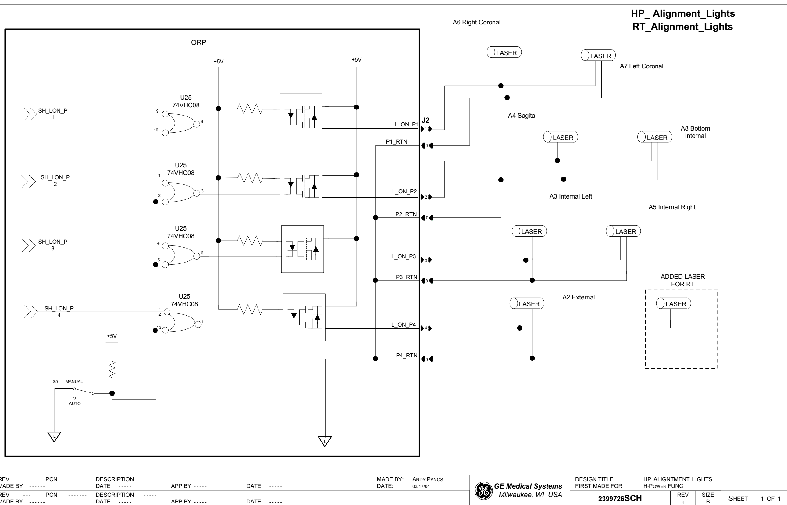
Figure 4-1 2399726 Sheet 1, Rev 1
