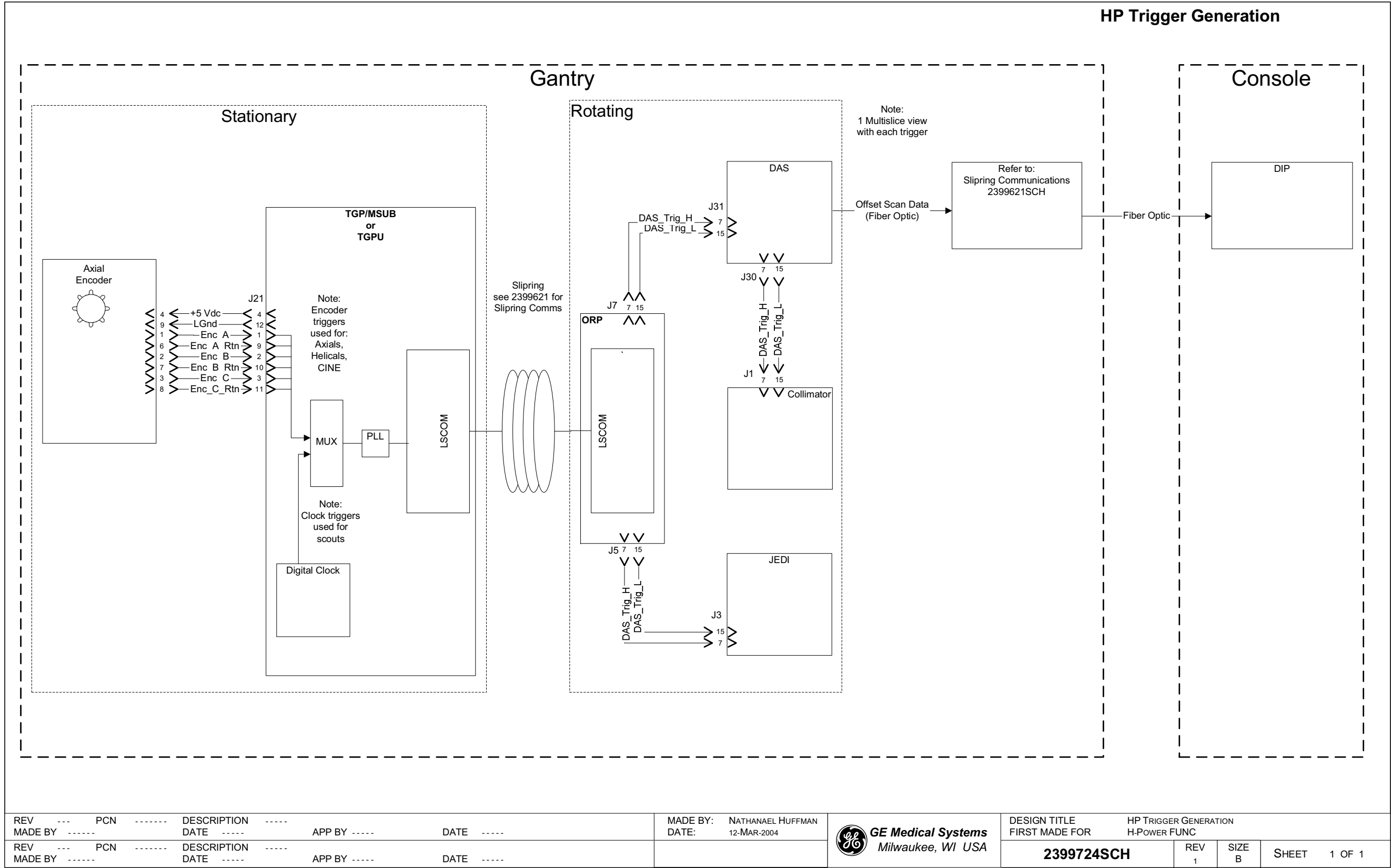
Figure 3-1 2399724 Sheet 1, Rev. 1
