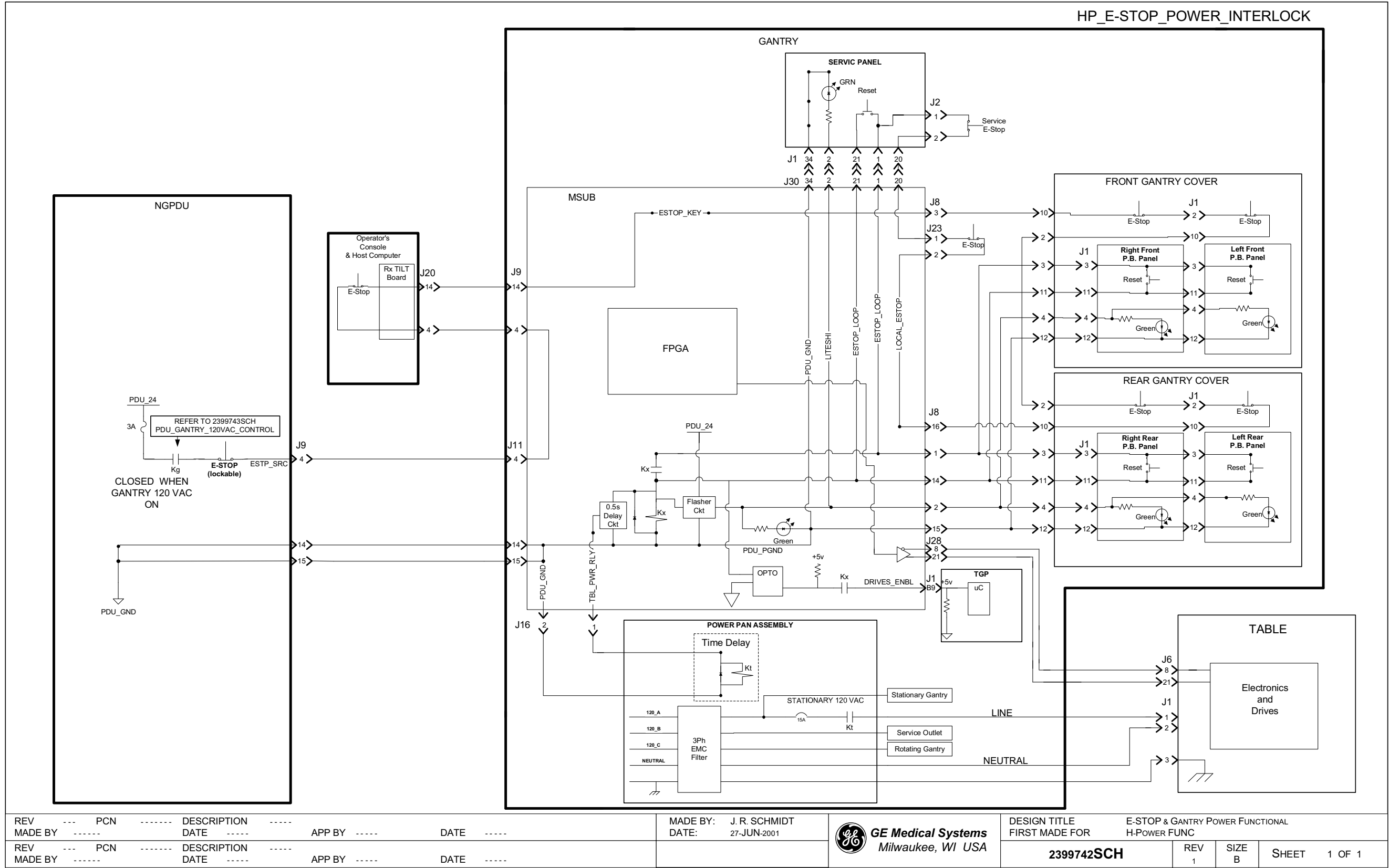
Figure 8-1 2399742 Sheet 1, Rev. 1
