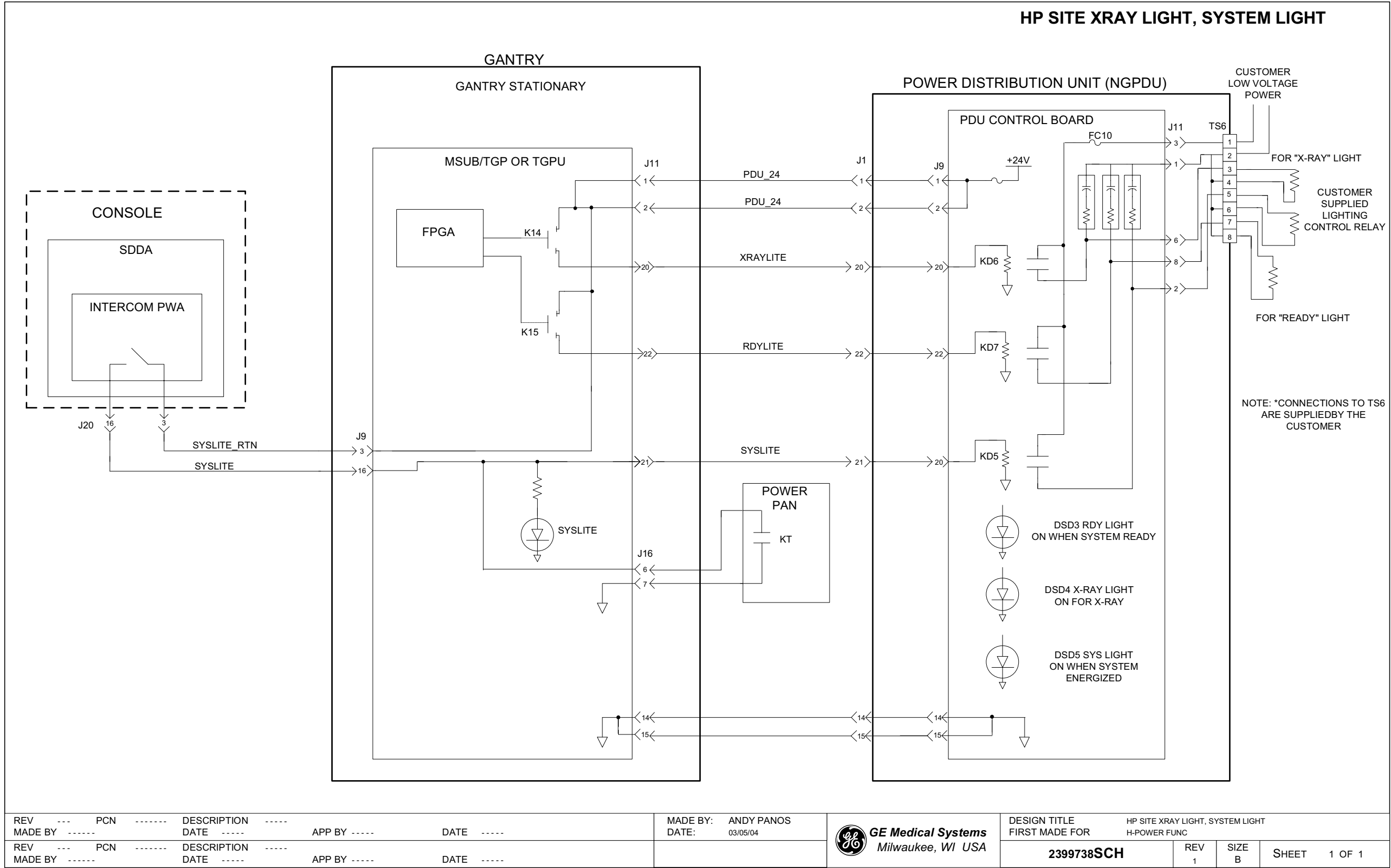
Figure 6-5 2399738 Sheet 1, Rev. 1
